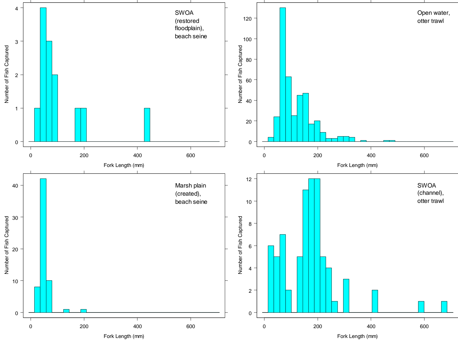
Figure 5-1. Size distribution for striped bass by habitat type and gear type, 2002-2005, Napa River FMP.
