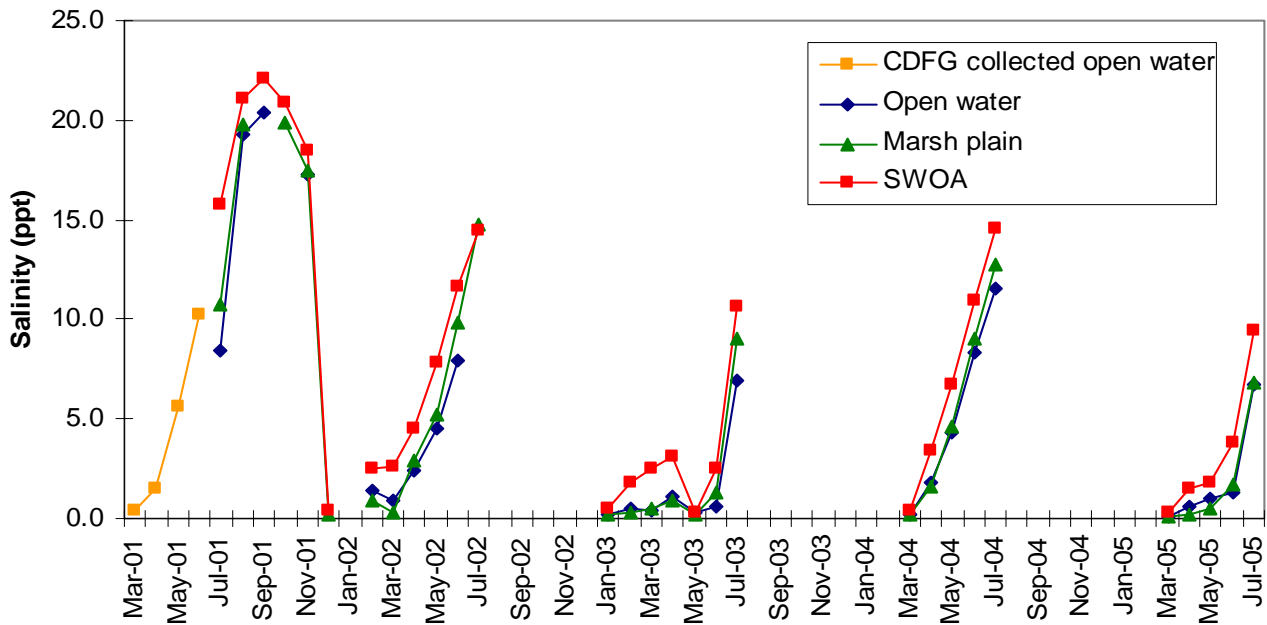
Figure A-8. Average salinity in SWOA, marsh plain, and open water habitats in the Napa River Project area, at the time of sampling in 2001–2005.
