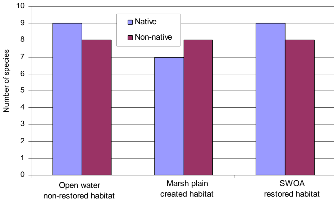
Figure 3-4. Number of species captured by habitat type in the Napa River Project area in 2005.
